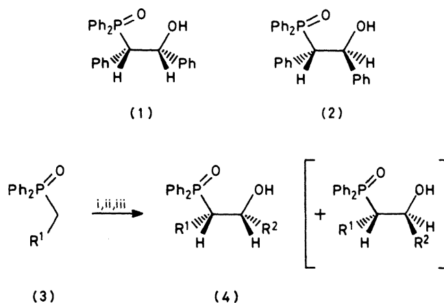
Scheme 1. Reagents: i, BuLi, 0^\circ\text{C} ; ii, \text{R}^2\text{CHO} , -78^\circ\text{C} ; iii, \text{H}_2\text{O} , -78 \rightarrow 0^\circ\text{C}
